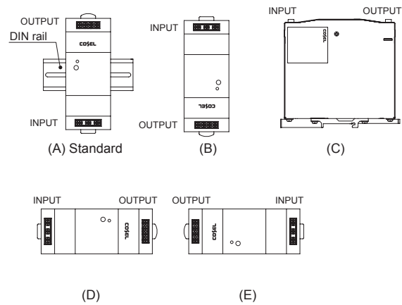
Fig.4.1 Mounting orientation
