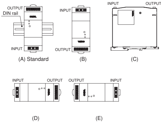
Fig.5.1 Mounting orientation
