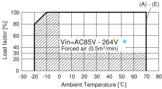
Fig.5.20 Derating curve depend on ambient temperature
