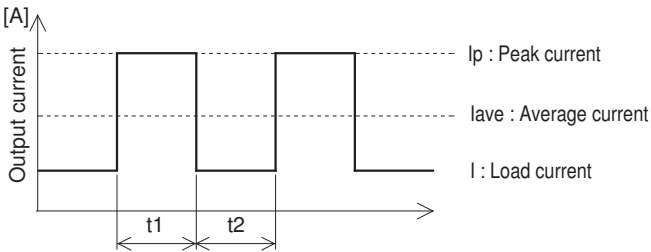
Fig.3.1 Peak current
